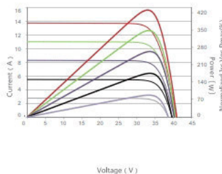
Current-Voltage & Power-Voltage Curves (430W)
